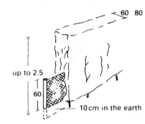
㉑ Hedge with wire netting
